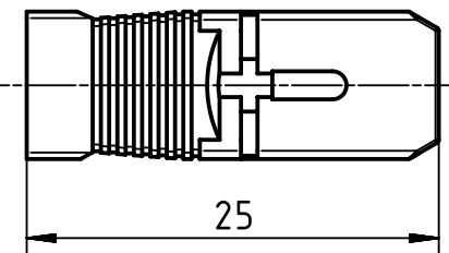
Crimping sleeve and boot for cable diameter Ø2,4 - Ø2,8 mm
