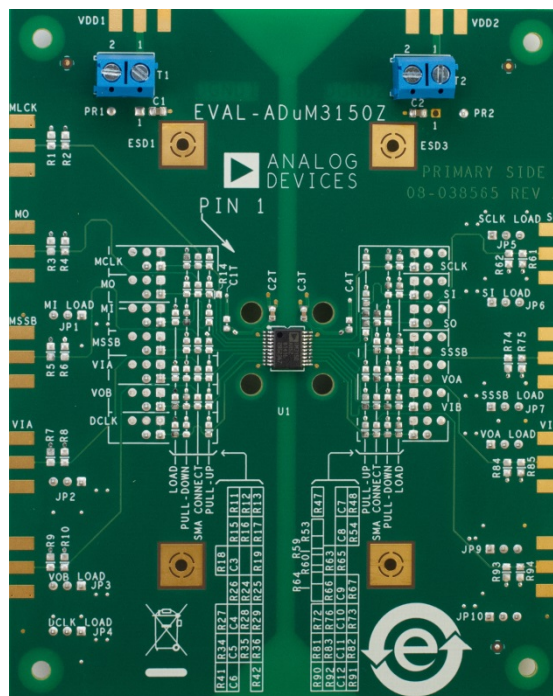
Figure 1. EVAL-ADuM3150Z Evaluation Board
