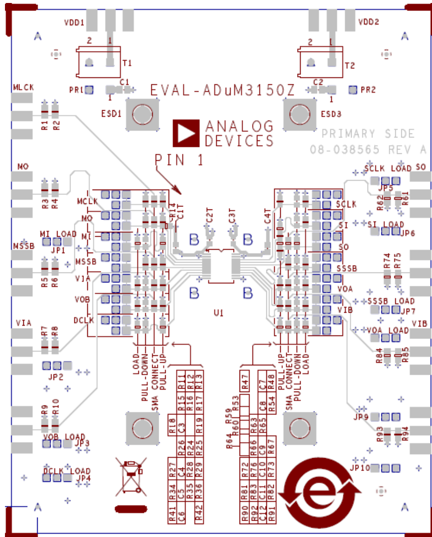
Figure 5. Top Side Layout
